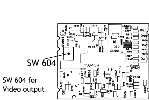
Fig. 37. Switches on PK8404.
