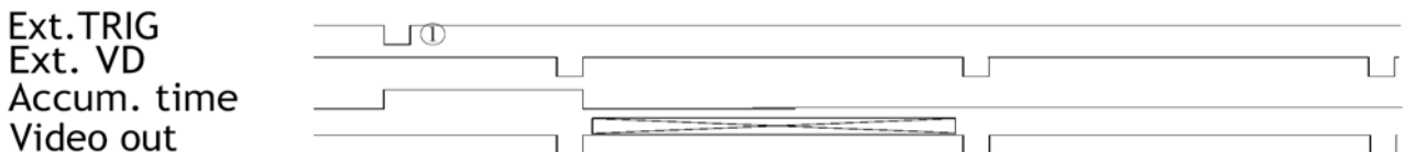
Fig. 24. Start stop interlaced frame integration
