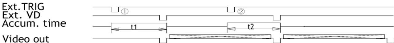
Fig. 25. Start stop non-interlaced field integration
