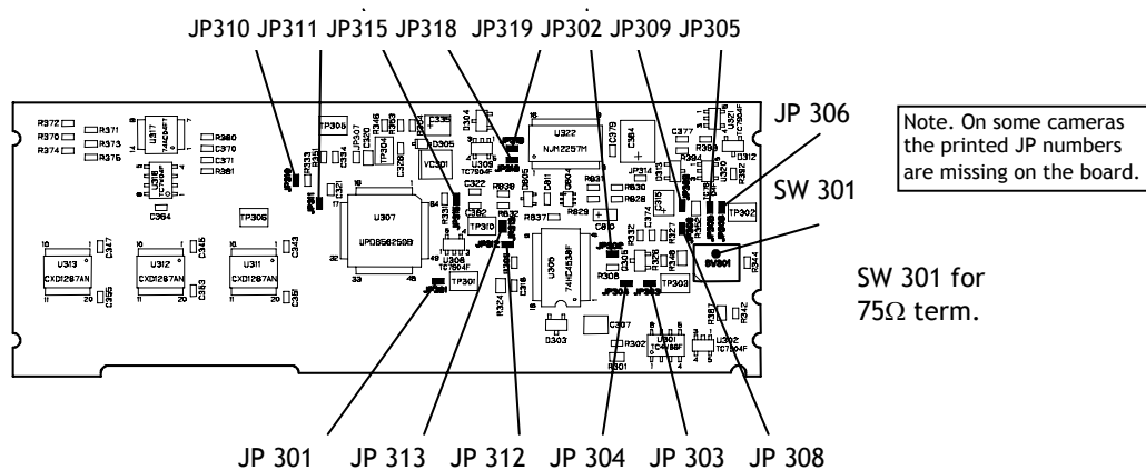
Fig. 36. Jumpers and switches on PK8407.
