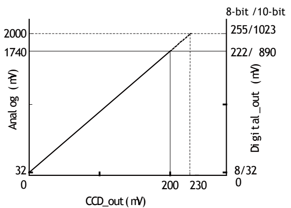
Fig.8 Video output
