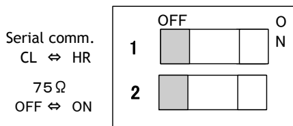
Fig.3 DIP switch
