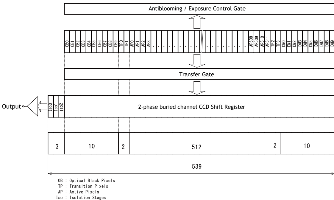
Fig.10 Sensor layout
