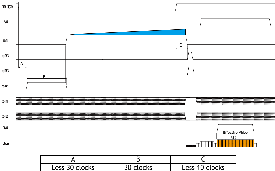
Fig. 18 Pulse Width Control mode
