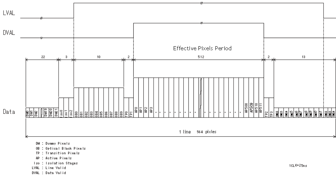
Fig.11 Video output timing
