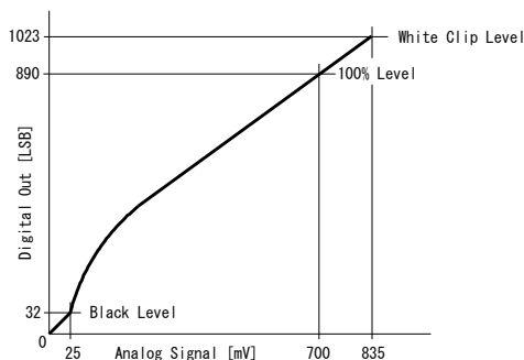
Fig.19 LUT characteristics
