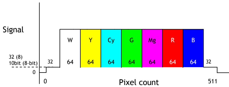
Fig. 21 Color bar test pattern
