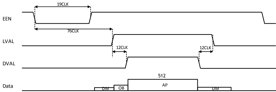
Fig.13 Detail of No-shutter with internal line rate generator
