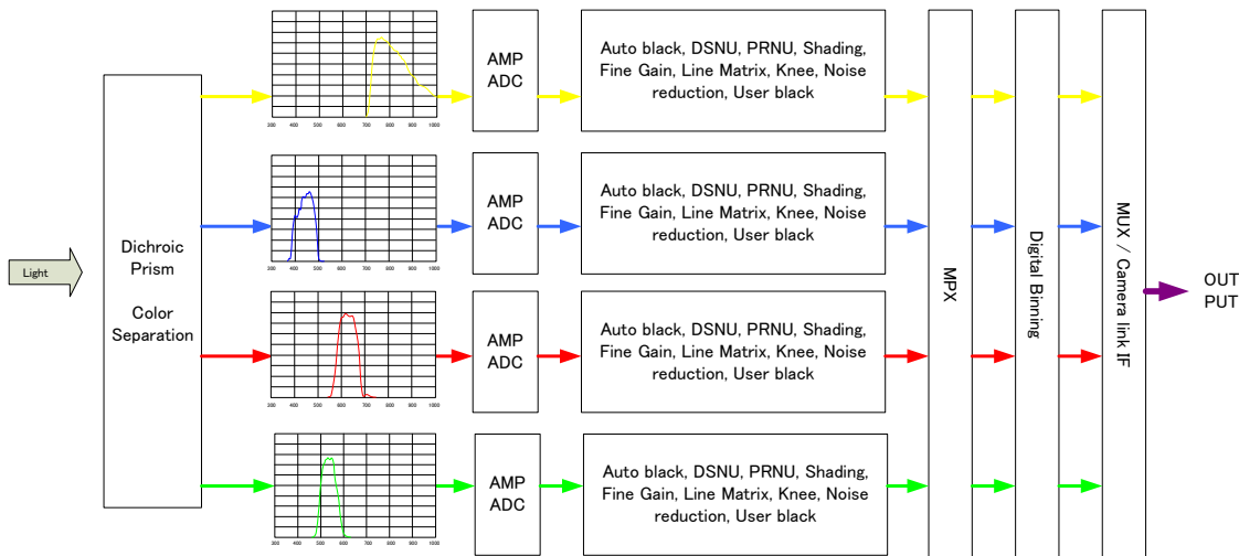
Fig.9 Signals flow
