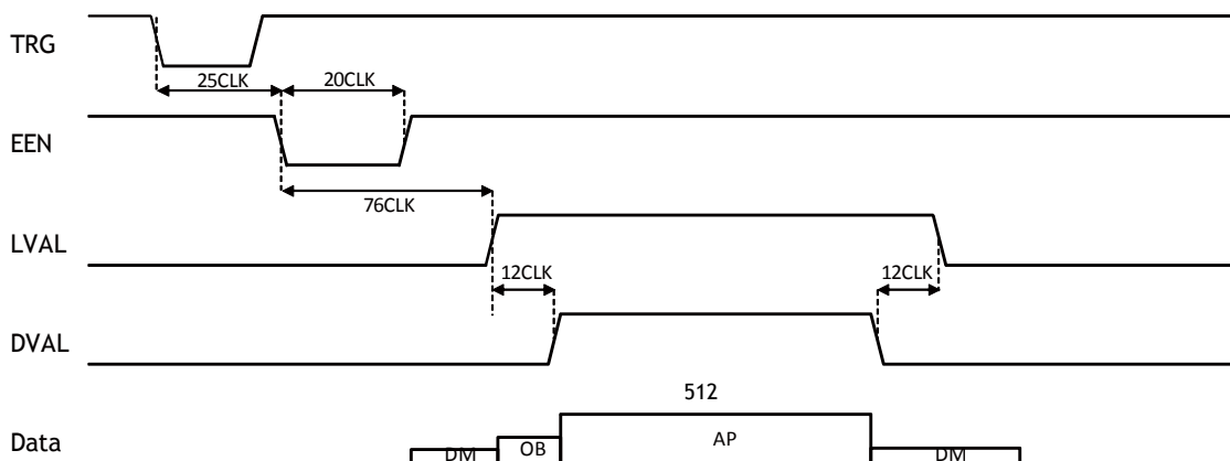
Fig. 15 Detail of No-shutter with external trigger
