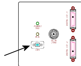
Fig.20 Rear panel
