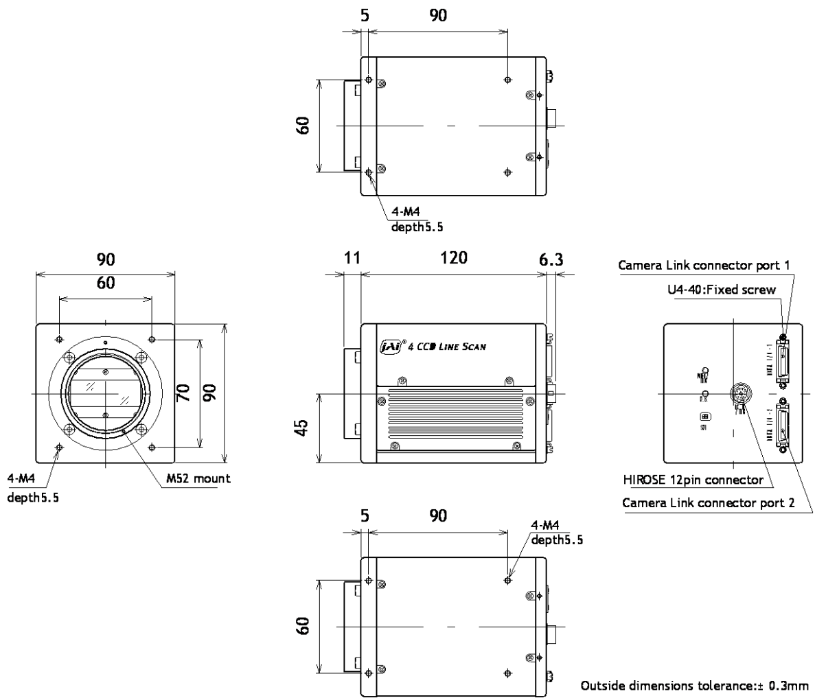
Fig.25 External Appearance and Dimensions for M52 mount
