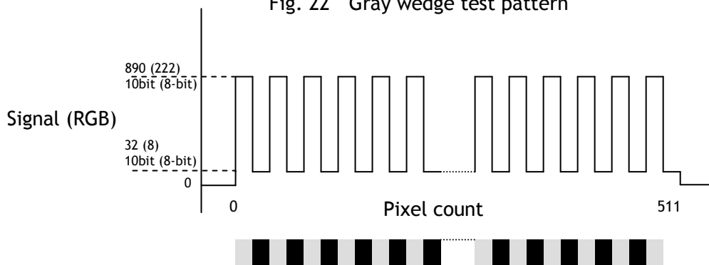
Fig. 23 Gray bars test pattern
