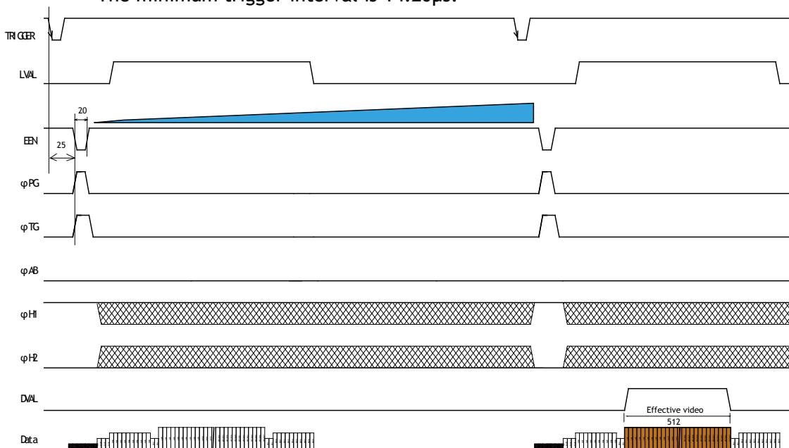
Fig. 14 No-Shutter mode with external trigger
