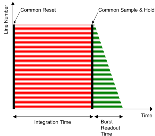
Figure 10. Global Shutter Operation
